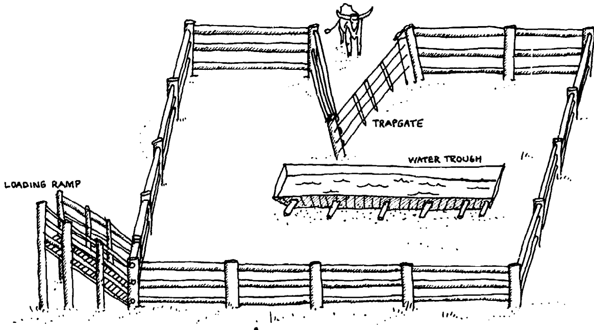
FIG. 5.22: TRAPIYARD - WATER TROUGH ATTRACTS FERAL HERBIVORES IN DROUGHT.
