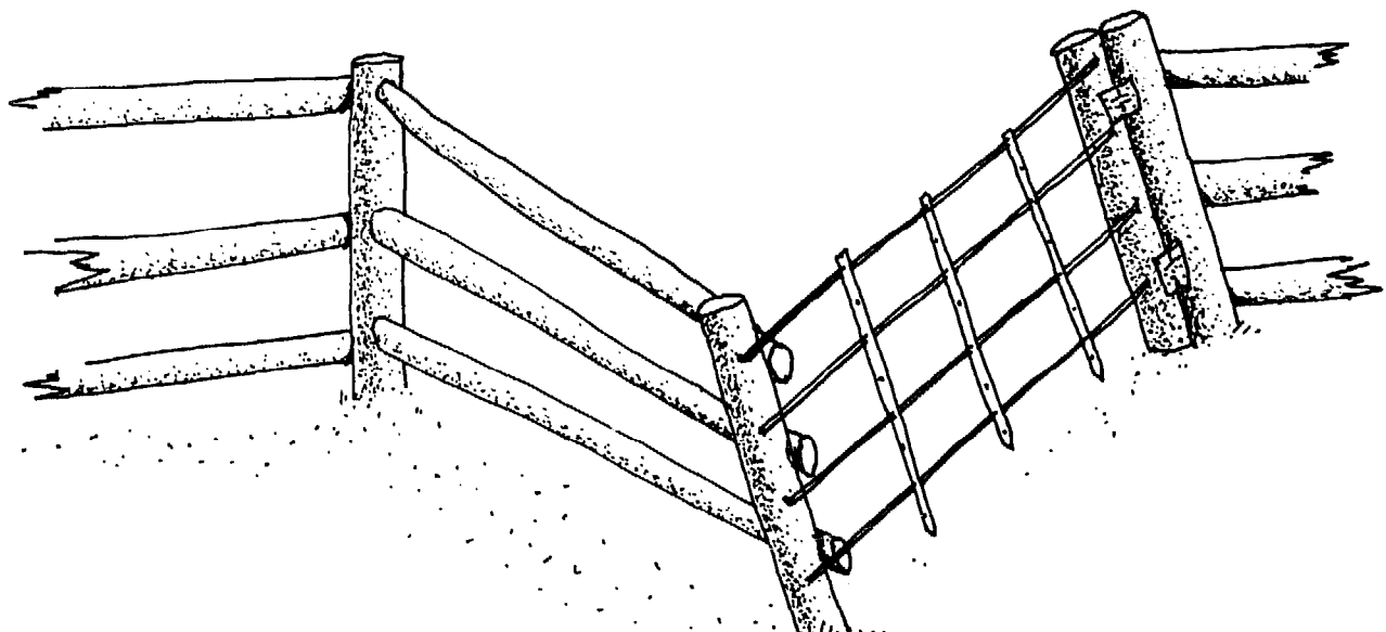
FIG. 5.22: TRAPIYARD - WATER TROUGH ATTRACTS FERAL HERBIVORES IN DROUGHT.
